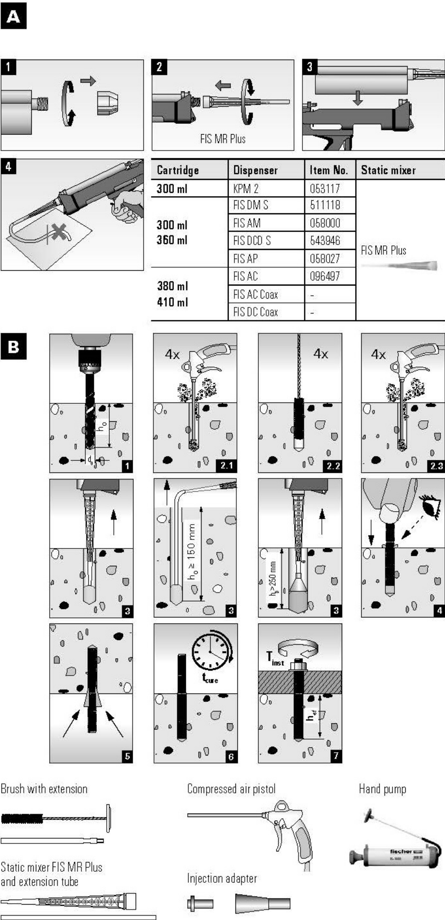
FIGURE 3—FIS V / FIS V PLUS INSTALLATION INFORMATION (Continued)
