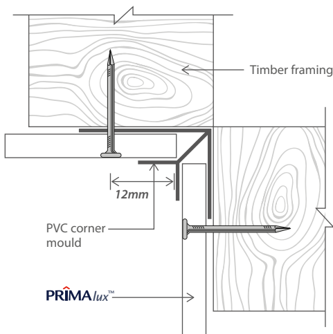
Figure 34: Internal Corner
