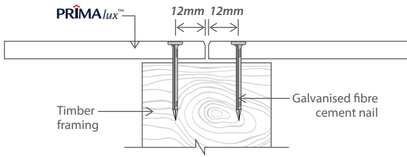
Figure 32: Butt Joint
