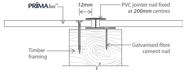
Figure 33: PVC Joint
