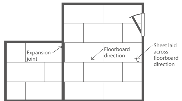
Figure 36: Underlay Orientation
