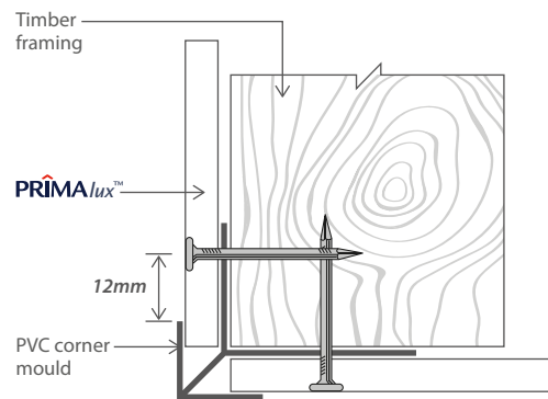
Figure 35: External Corner
