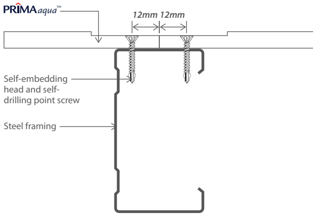
Figure 2: Fixing to Steel Support
