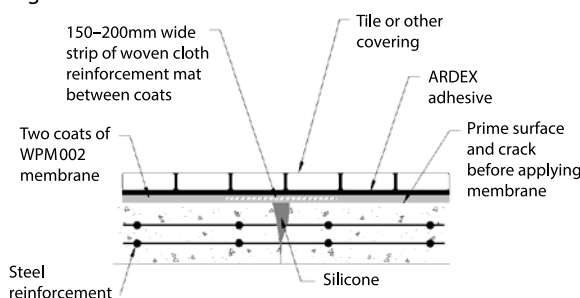
Fig.3 – Crack treatments
